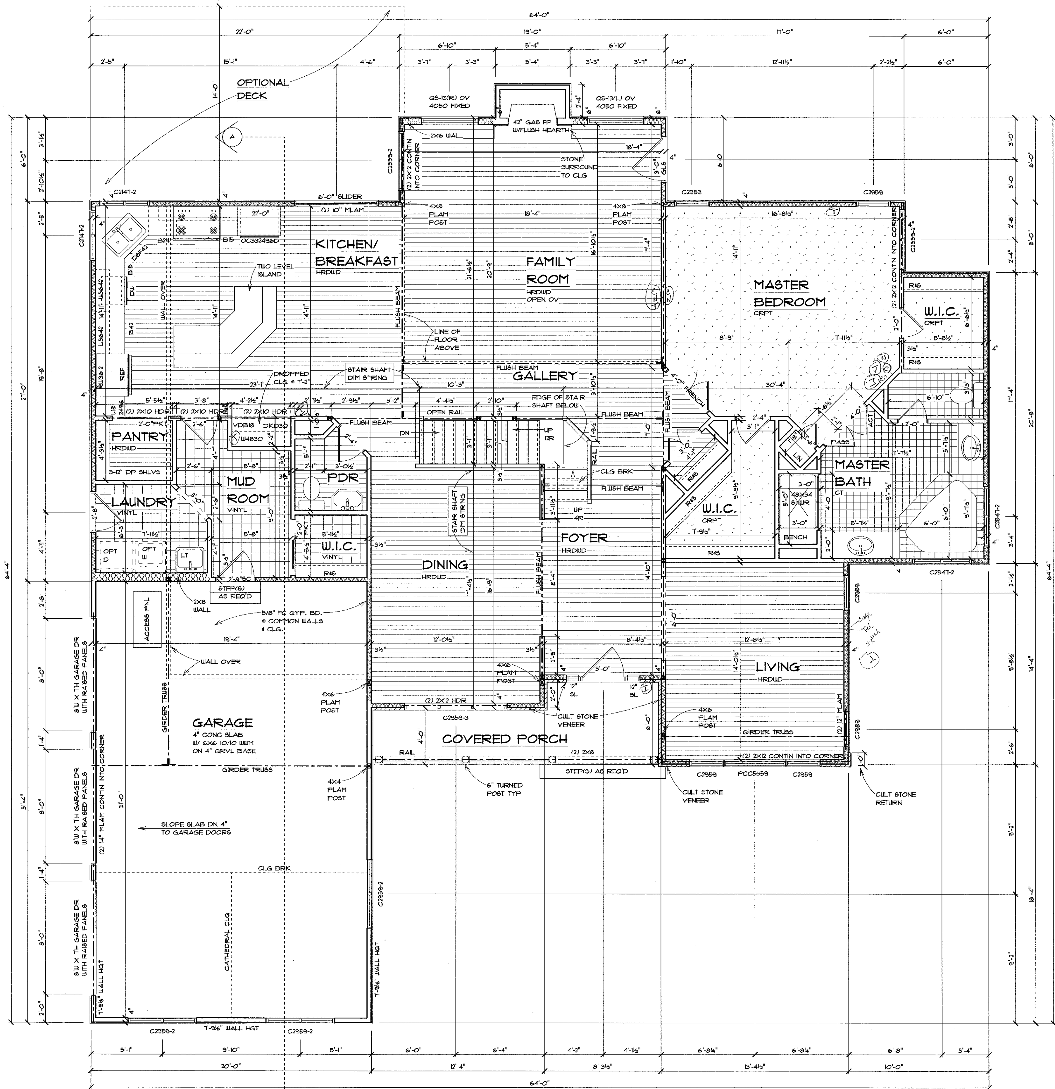
FIRST FLOOR PLAN APPROX 2131 SQ FT FIRST FLOOR APPROX 985 SQ FT SECOND FLOOR APPROX 3122 SQ FT TOTAL
